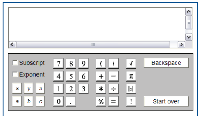
Equation Editor
