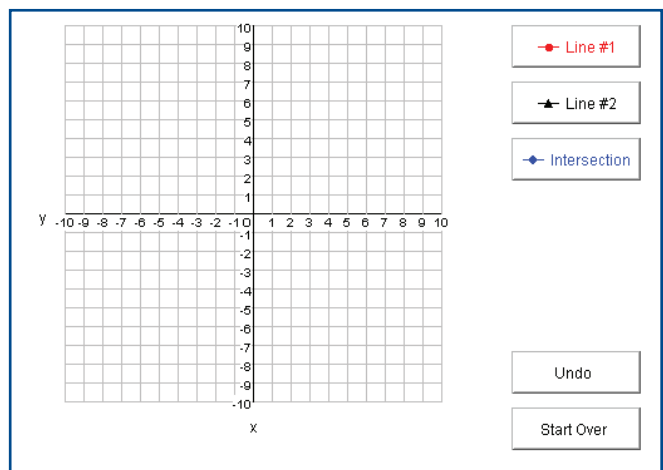
Graph Editor
